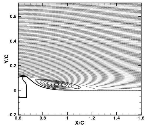
No-Flow, NASA-fun2d-sa-u2:
