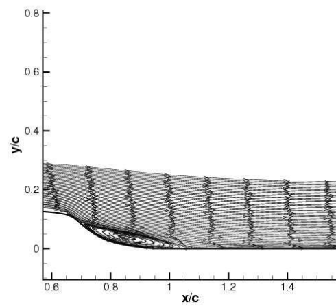
Suction, CIRA-zen-sst-oj-3:
