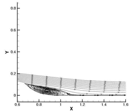
Suction, AFRL-fdl3di-ke-c4:
