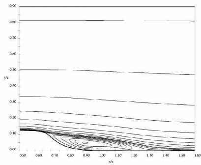
No-Flow, UAZ-dns-3d:
