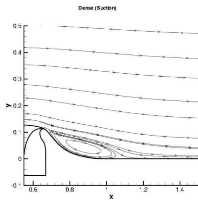
Suction, UK-ghost-sst-1:
