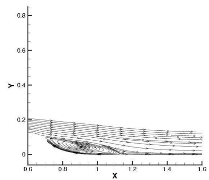
Suction, AFRL-fdl3di-ke-f2:
