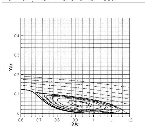
No-Flow, CTR-fluent-sa-1:
