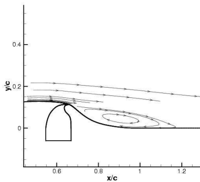
No-Flow, CTR-fluent-sa-1:
