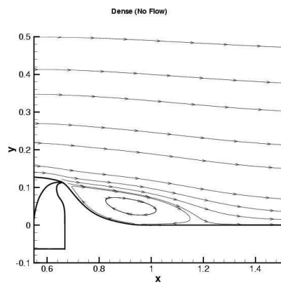
No-Flow, UK-ghost-sst-1:
