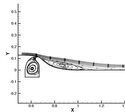
Suction, UMD-rans-sa-roe-2:
