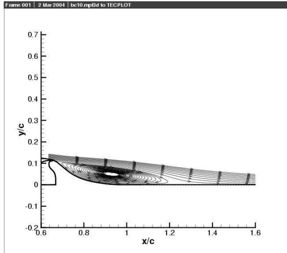
No-Flow, NASA-rans-sst-weno5:
