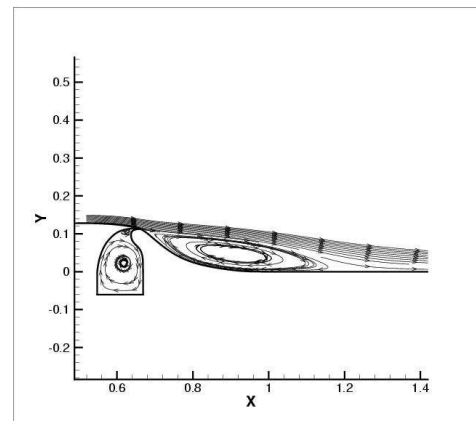
No-Flow, UMD-rans-sa-roe-2:
