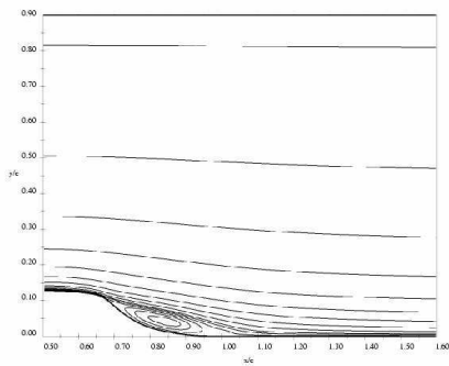
Suction, UAZ-dns-3d:
