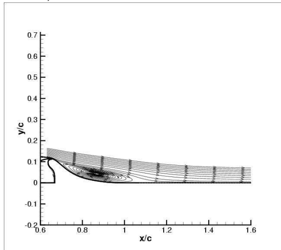
Suction, NASA-rans-sst-weno5:
