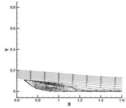
No-Flow, AFRL-fdl3di-ke-c4:
