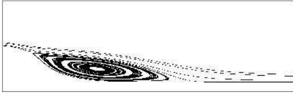
No-Flow, AZ-cobalt-sa-1-blr:
