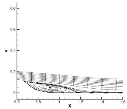
No-Flow, AFRL-fdl3di-ke-f2:
