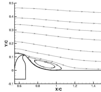
Suction, UMD-rans-sa-cent-2:
