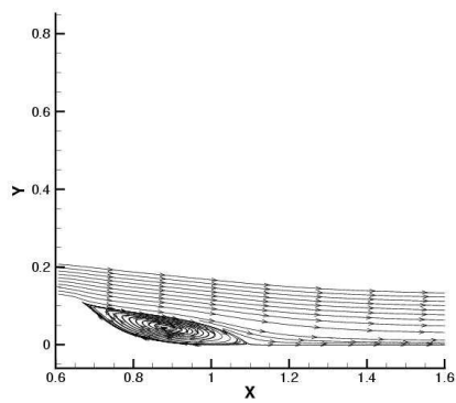
Suction, AFRL-fdl3di-ke-c4-3d:
