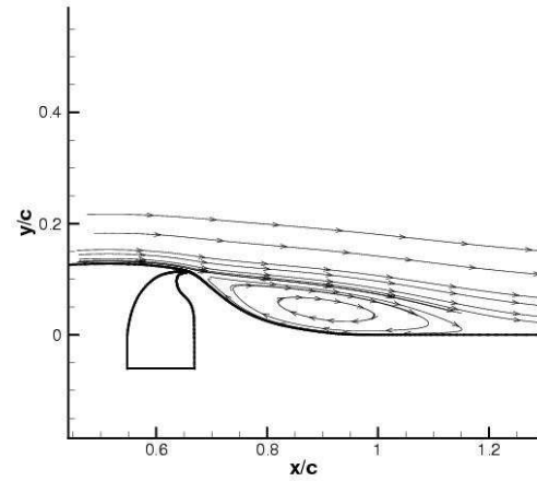
No-Flow, CIRA-zen-sst-3:
