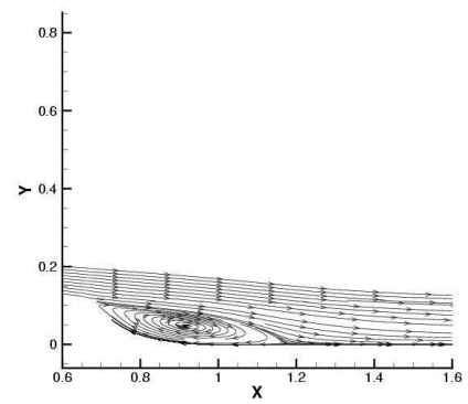
No-Flow, AFRL-fdl3di-ke-f2:
