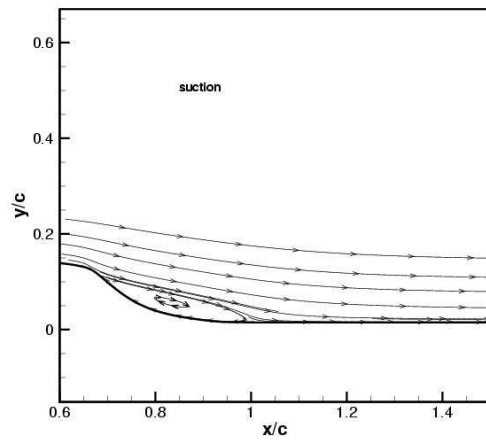
Suction, NASA-rans-sst-weno5:
