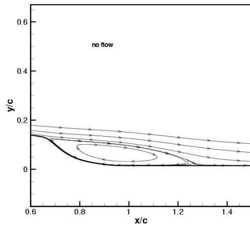
No-Flow, NASA-rans-sst-weno5:
