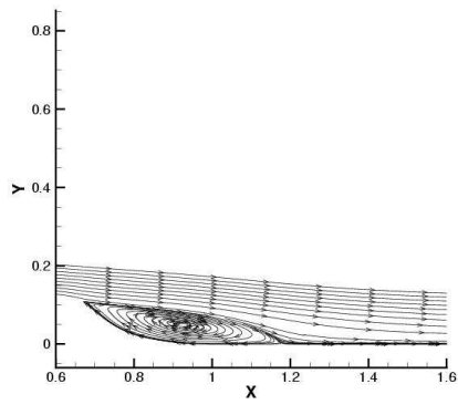
No-Flow, AFRL-fdl3di-ke-c4-3d:
