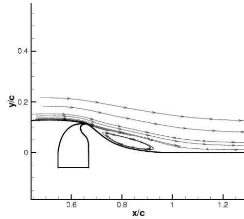
Suction, CIRA-zen-sst-nj-3:
