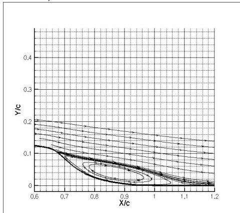
Suction, CTR-fluent-sa-1:
