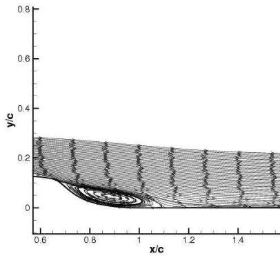
No-Flow, CIRA-zen-sst:
