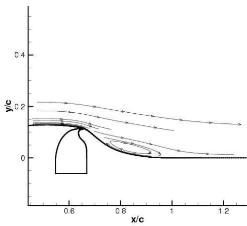
Suction, CTR-fluent-sa-1:
