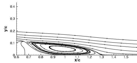
No-Flow, NASA-cfl3d-sst-2:
