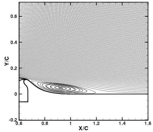
No-Flow, NASA-fun2d-sa-u2:
