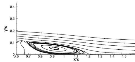
No-Flow, NASA-cfl3d-sa-top-5:
