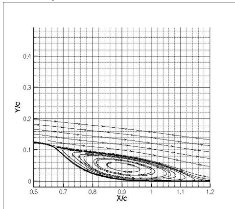
No-Flow, BOEING-overflow-sst:
