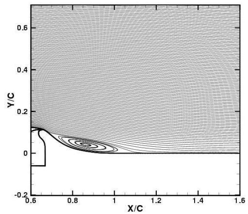
Suction, NASA-fun2d-sa-u2:
