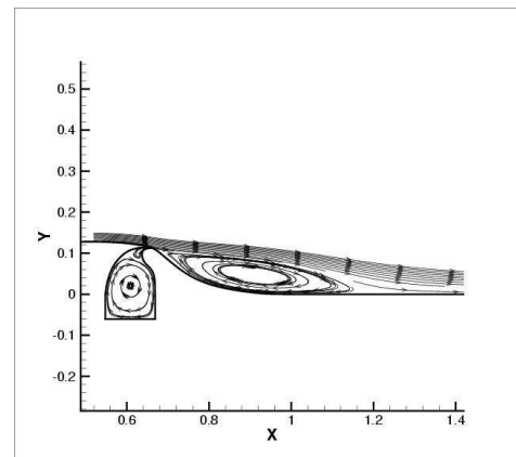
No-Flow, UMD-rans-sa-cent-2:
