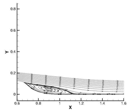
Suction, AFRL-fdl3di-ke-f2:
