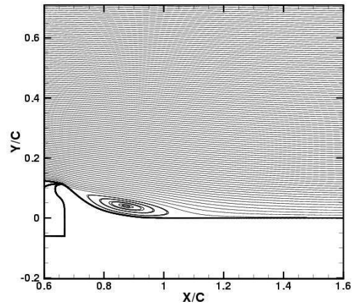
Suction, NASA-fun2d-sa-u2:
