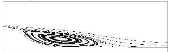
No-Flow, AZ-cobalt-sst-1c:
