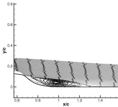
No-Flow, NASA-cfl3d-sa-1:
