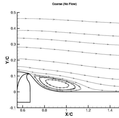
No-Flow, UK-ghost-sst-2:
