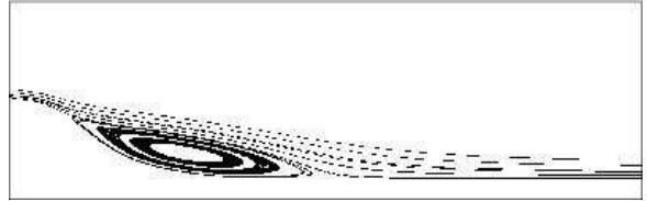
Suction, AZ-cobalt-sa-2:
