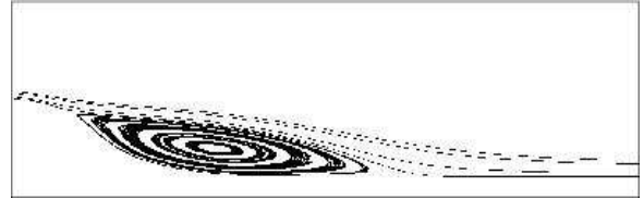
No-Flow, AZ-cobalt-sa-2:
