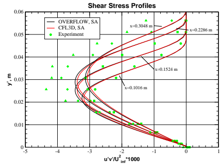
Figure 11.5: Turbulent shear stress profiles, SA model.
