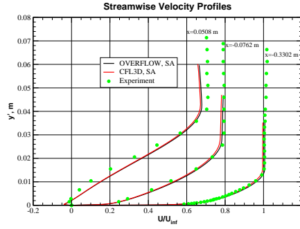
Figure 11.4: Streamwise velocity profiles, SA model.
