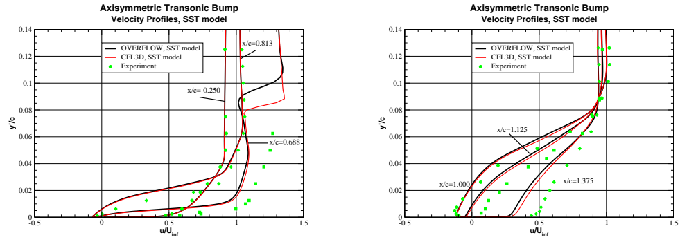
Figure 12.7: Streamwise velocity profiles, SST model.
