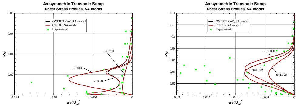
Figure 12.5: Turbulent shear stress profiles, SA model.
