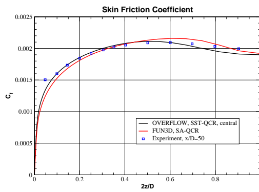
Figure 19.11: Skin friction and crossflow velocity, SST-QCR model.
