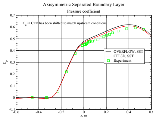
Figure 11.6: Pressure coefficient and skin friction, SST model.
