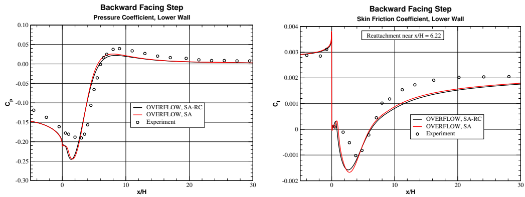
Figure 14.12: Pressure coefficient and skin friction, SA and SA-RC models, finest grid.
