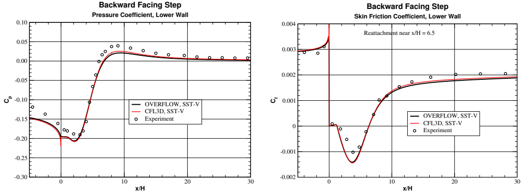
Figure 14.9: Pressure coefficient and skin friction, SST-V model.
