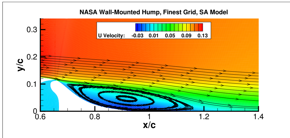
Figure 17.10: Streamlines and u -velocity contours, SA model.
