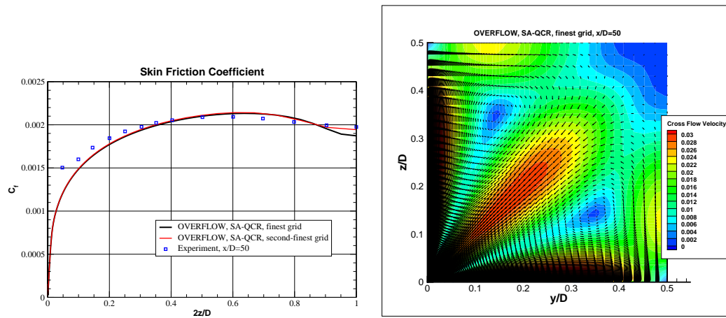
Figure 19.13: Skin friction and crossflow velocity, SA-QCR model, finest grid.
