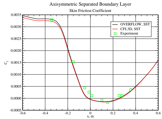
Figure 11.6: Pressure coefficient and skin friction, SST model.
