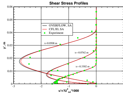
Figure 11.5: Turbulent shear stress profiles, SA model.
