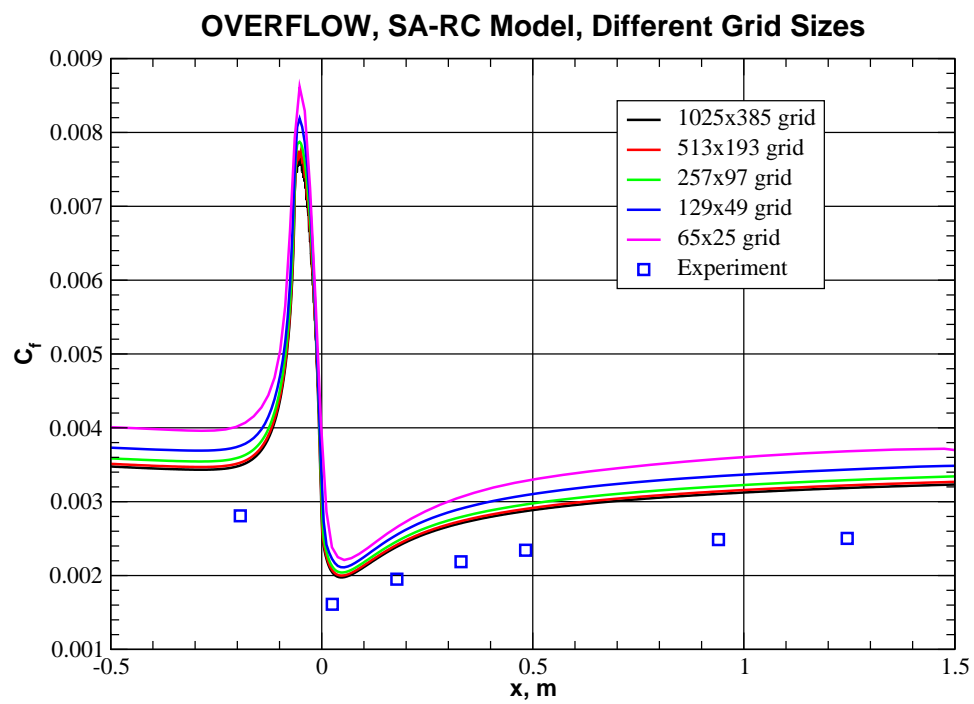
Figure 16.28: Lower wall skin friction, SA-RC, varying grid dimensions.
