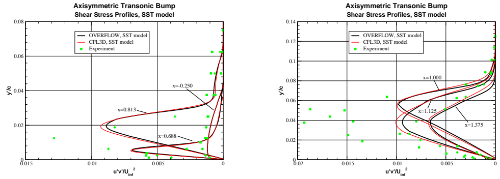
Figure 12.8: Turbulent shear stress profiles, SST model.
