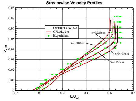
Figure 11.4: Streamwise velocity profiles, SA model.
