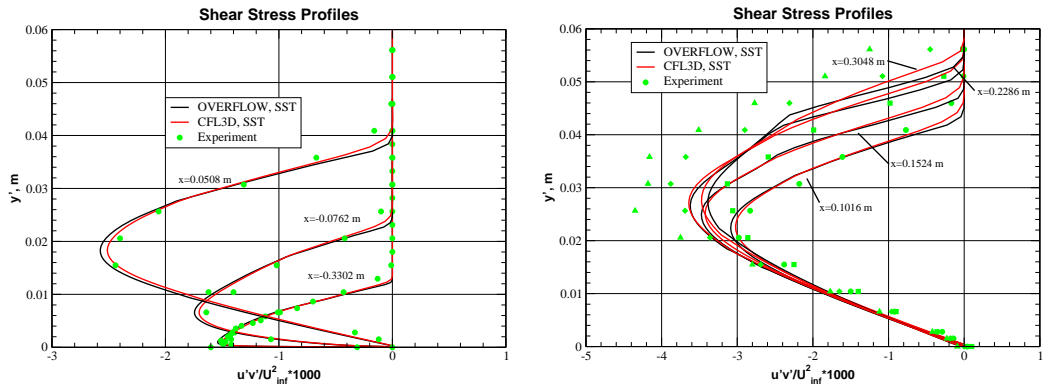
Figure 11.8: Turbulent shear stress profiles, SST model.
