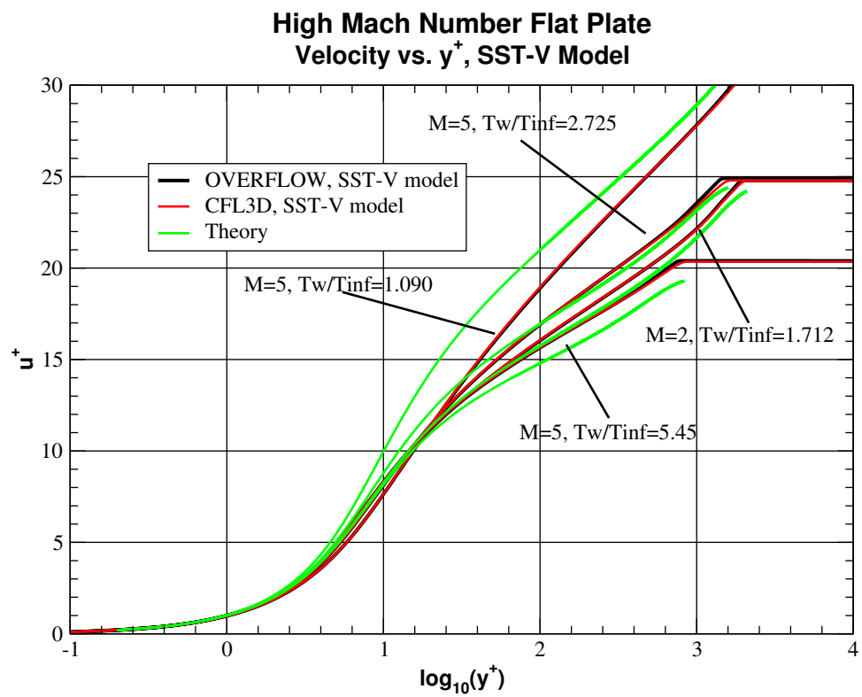
Figure 13.7: u^+ , SST-V model.
