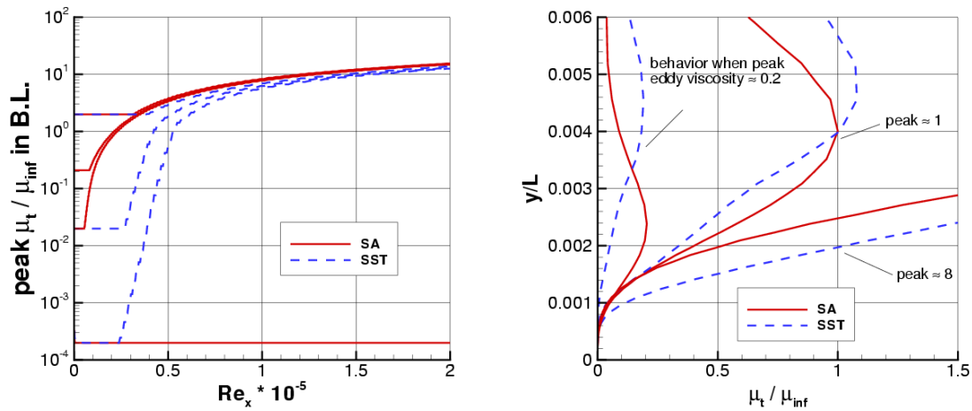
Figure 8. Eddy viscosity over flat plate, M = 0.2 , medium grid; (a) peak value; (b) vertical profile at locations where peak \mu_t / \mu_{\infty} \approx 0.2, 1.0, \text{ and } 8.0 .
